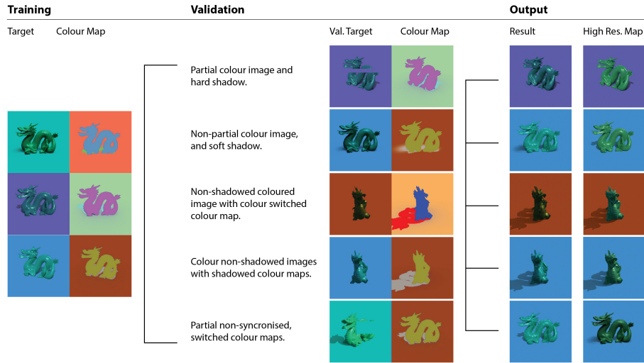
Fig. 6: Phase two of the third set focused on the interpretation of coloured shadows, since shadows are darker values of colours and not gray values.
