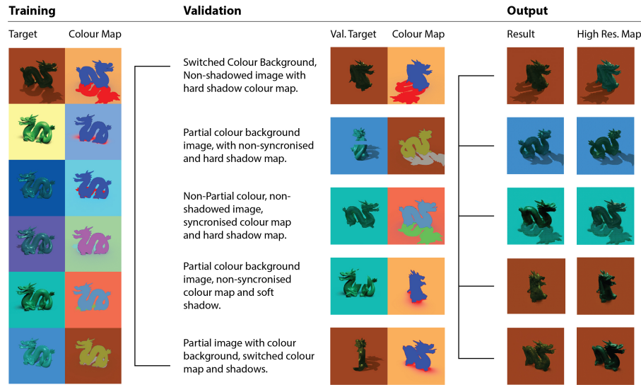
Fig. 7: In the third and final phase of the third set, we pushed the code to its limits by switching targets, colour background and colour maps.
